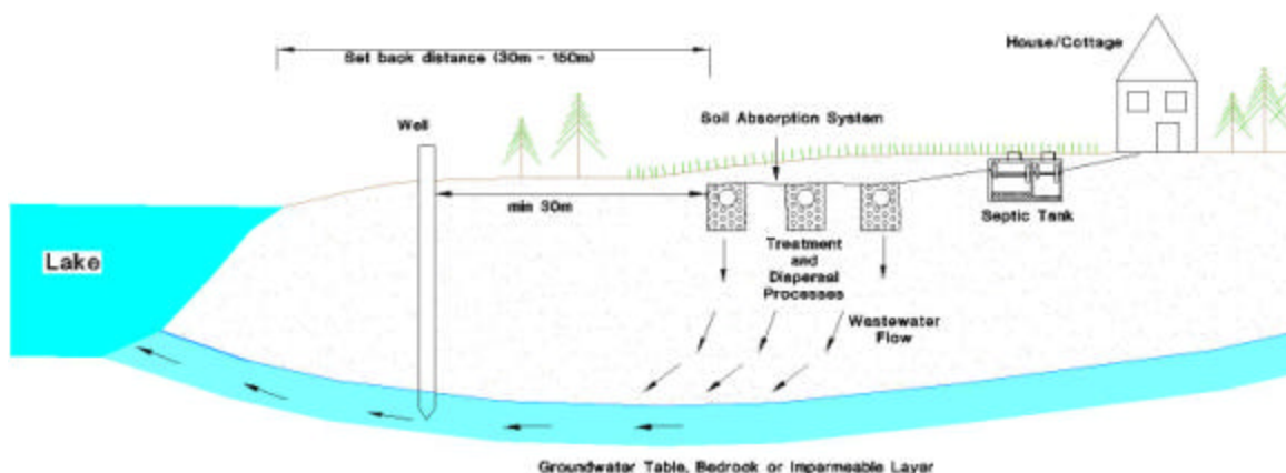
Figure #5: Onsite treatment and dispersal of wastewater in a lakeshore environment
