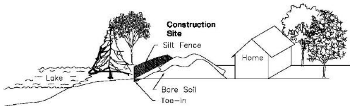
Figure #3: A Silt Fence in Use During Construction.
